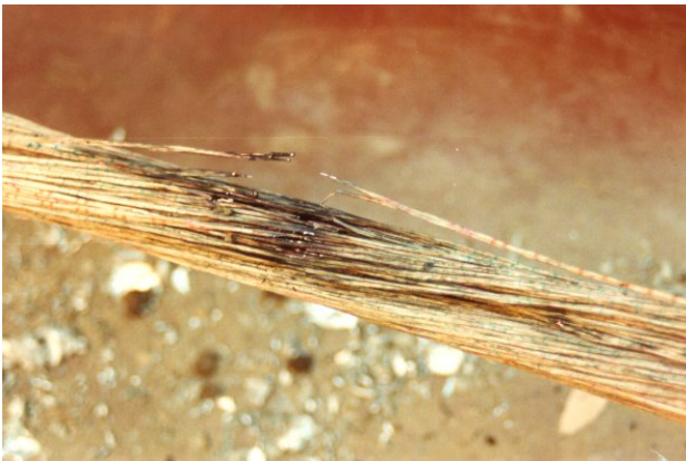
Photo 2: Damaged Telecom Cable
